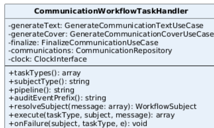
Figura 52: Classe — CommunicationWorkflowTaskHandler
