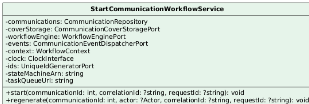
Figura 55: Classe — StartCommunicationWorkflowService
