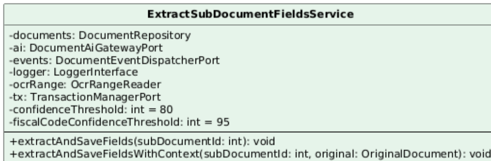
Figura 24: Classe — ExtractSubDocumentFieldsService
