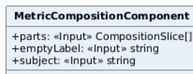
Figura 117: Classe — MetricCompositionComponent
