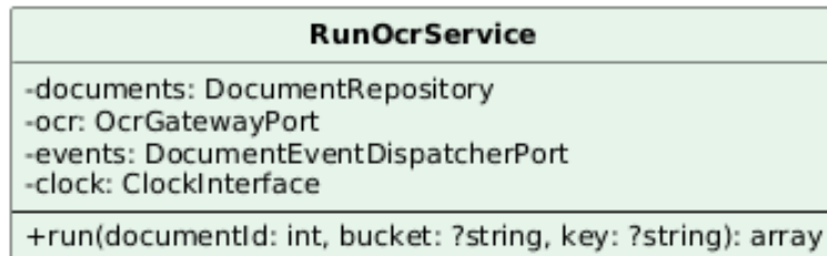
Figura 22: Classe — RunOcrService
