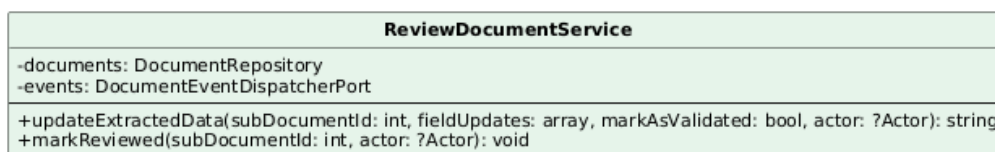
Figura 28: Classe — ReviewDocumentService
