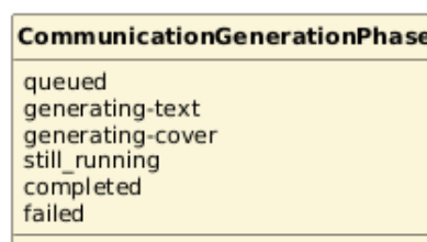
Figura 94: Tipo — CommunicationGenerationPhase
