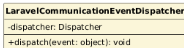
Figura 74: Classe — LaravelCommunicationEventDispatcher
