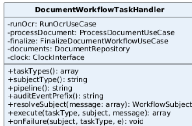
Figura 17: Classe — DocumentWorkflowTaskHandler
